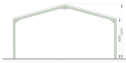
NORTH ELEVATION (SOUTH ELEVATION IDENTICAL)
